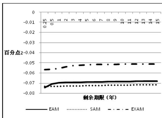
图 6 二阶矩样本期内预测误差均值 Fig 6 Mean value of in-sample Forecast errors of second moment
