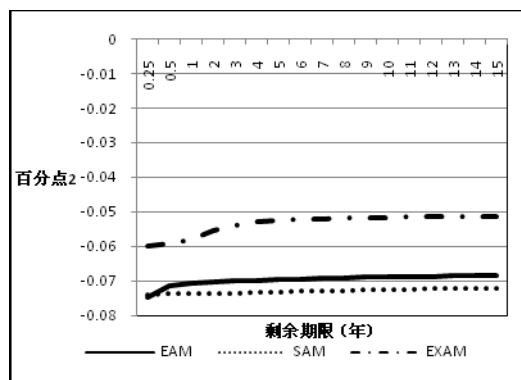
图 7 二阶矩样本期外预测误差均值 Fig 7 Mean value of out-of-sample Forecast errors of second moment
