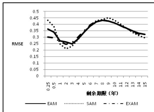
图 5 样本期外一阶矩预测误差 RMSE Fig 5 RMSE of out-of-sample Forecast errors of first moment
