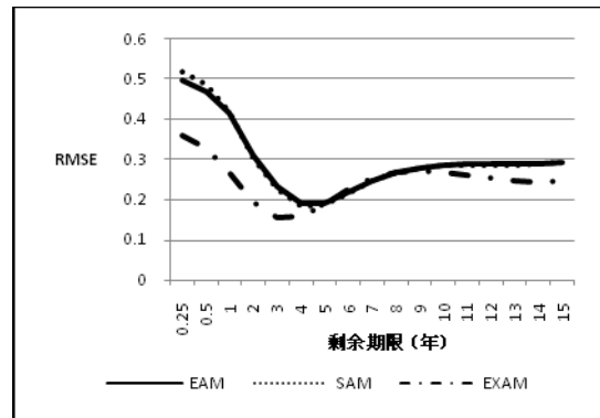
图 3 样本期内一阶矩预测误差 RMSE Fig 3 RMSE of in-sample Forecast errors of first moment
