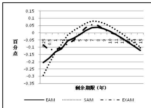
图 4 样本期外一阶矩预测误差均值 Fig 4 Mean value of out-of-sample Forecast errors of first moment
