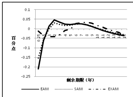
图 2 样本期内一阶矩预测误差均值 Fig 2 Mean value of in-sample Forecast errors of first moment
