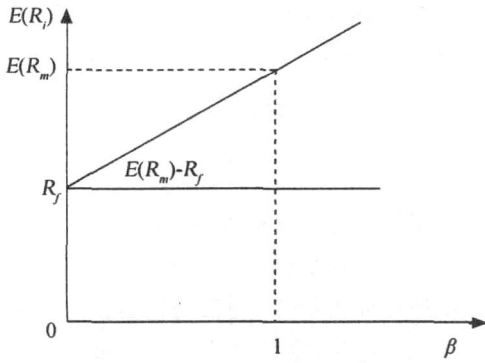
图1 均值-方差CAPM模型的证券市场线 Fig. 1 Security market line of Mean Variance CAPM
